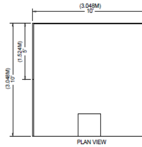
PLAN VIEW
